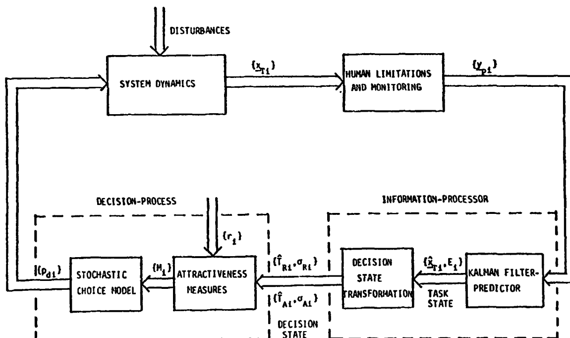
Fig. 3. DYNAMIC DECISION MODEL OF HUMAN TASK SELECTION PERFORMANCE
