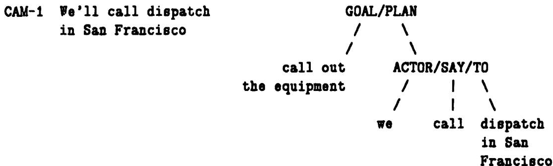
Figure 4: Addition of an ACTOR/SAY/TO Node
